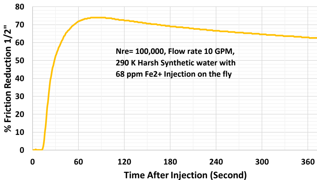
Figure 3. FR performance of TEXAN CATIONIC DPAM in 1/2"OD and 290K TDS Synthetic water with 68 ppm Fe2+ The above graph shows that Texan Cationic DPAM Slurry 2.5 lb. loading achieves around 73% Friction reduction in less than a minute of injection and exhibits good shear resistance under extremely harsh water conditions with good amounts of Divalent Cations, high specific gravity and low pH level.
