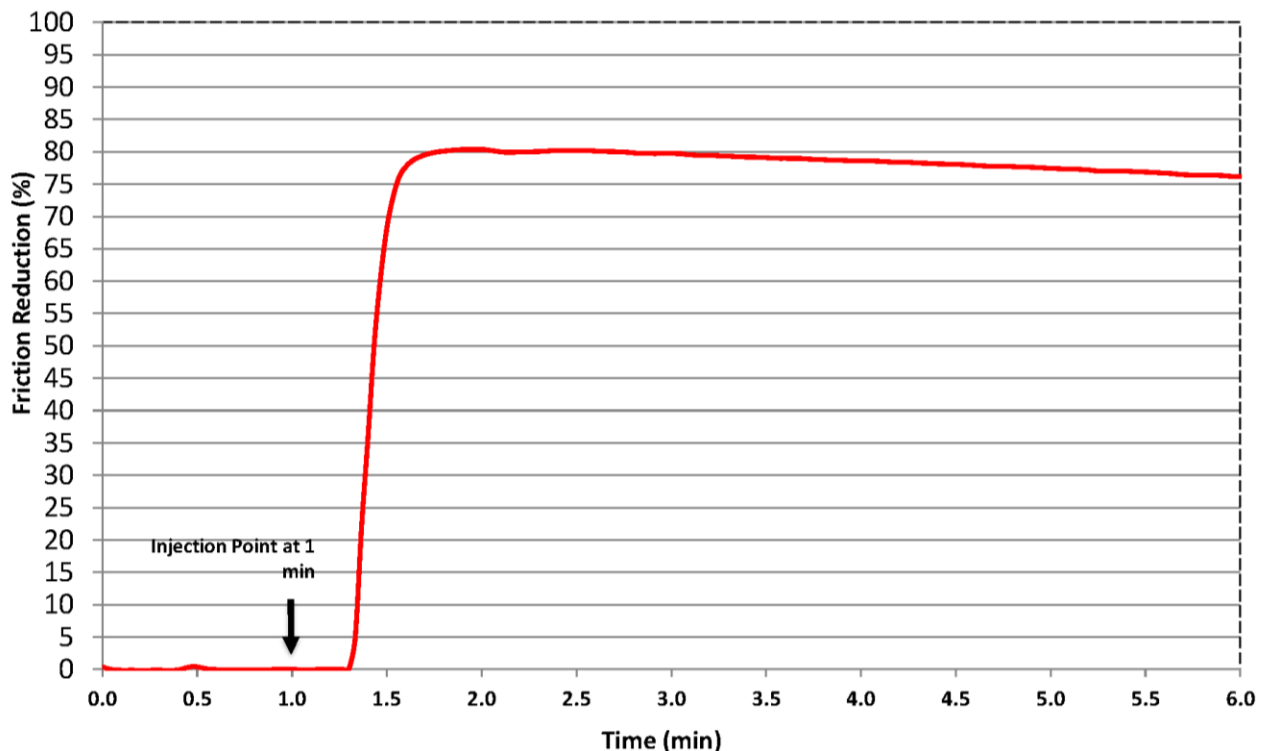
Figure 1. FR performance of TEXAN CATIONIC DPAM in 3/8"OD in 108 K TDS API brine at room temperature
