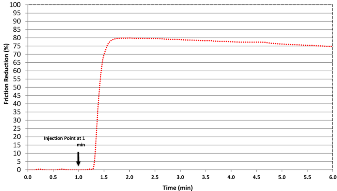
Figure 2. FR performance of TEXAN CATIONIC DPAM in 3/8"OD and 150K TDS Marcellus brine at room temperature
